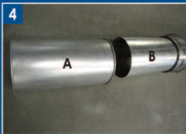
4 Debur cut and slide sleeve (A) over cut end of pipe (B).
